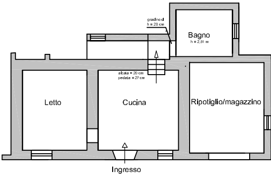
PIANO TERRA h = 2,50 m circa
